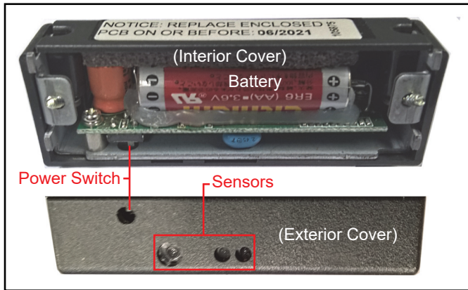
Figure 1 UBA® ICB® Assembly (Standard Cash Box)
